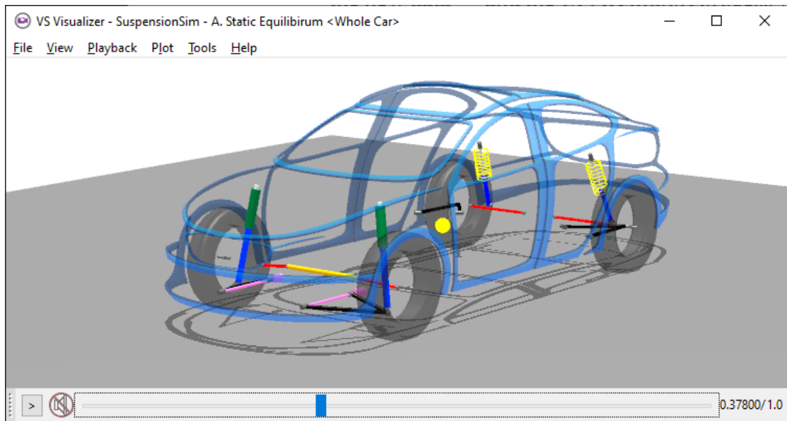
Figure 8. Updated "Whole Car" example, using the new car shape.
